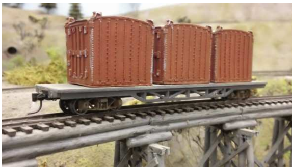
PJM wagon (steel) with steel truss frame
